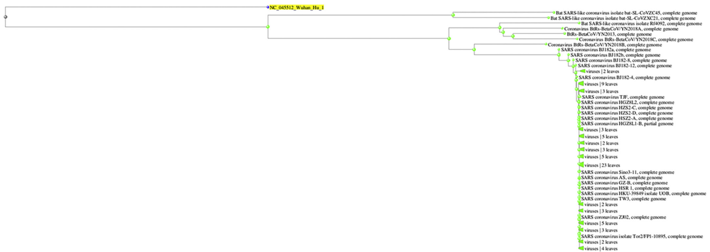
Fig. 2. Neighbor joining distance tree of the BLAST search results of the 2019-nCoV (NC_045512_Wuhan_Hu_1) sequence in the genomic region 10,901–22,830 of the alignment.
